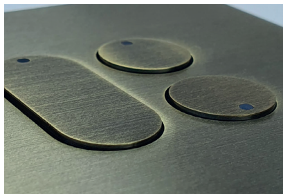
B4 KNX Radius BUTTON
