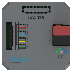
LXA - 138 8 Gang KNX Universal Push Button interface
