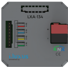
LXA - 134 4 Gang KNX Universal Push Button interface
