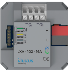
LXA - 102 - 16A 2 Gang Switch + 2 Digital KNX Actuator Flush-Mounted
